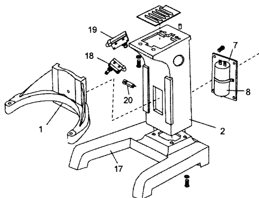
Figure 7 MACHINE SEAT, STAND AND HANDWHEEL TYPEBOWL LIFTER UINT
