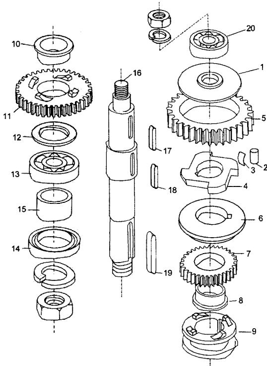
Figure 2 AXLE
